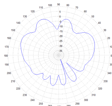
5500 MHz – Elevation Plot
