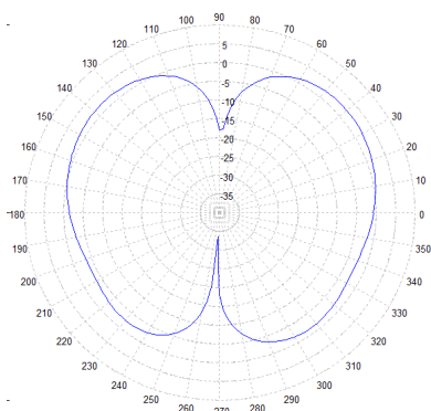
620 MHz – Elevation Plot
